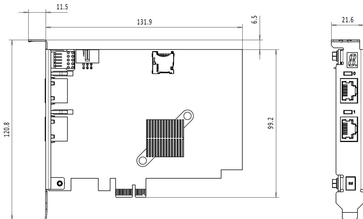
Dimensions ibaN-2E, dimensions in mm
